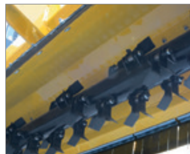
There is a lower suction effect thanks to the special Y-blades installed on the rotor and a variably adjustable working height of up to approx. 11 cm, meaning that reptiles and small organisms remain on the ground and do not come into contact with the Y-blades.
