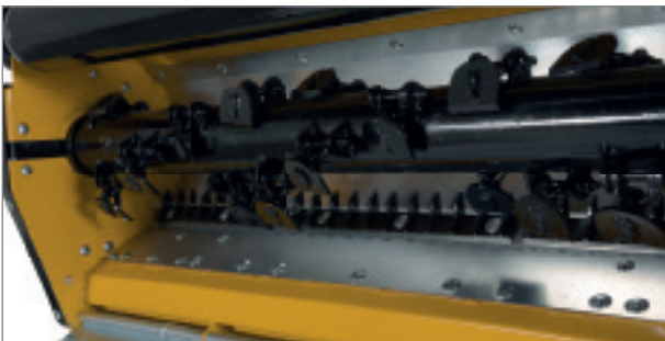
Wear insert for rough day-to-day usage by service providers and municipal authorities (optional).
